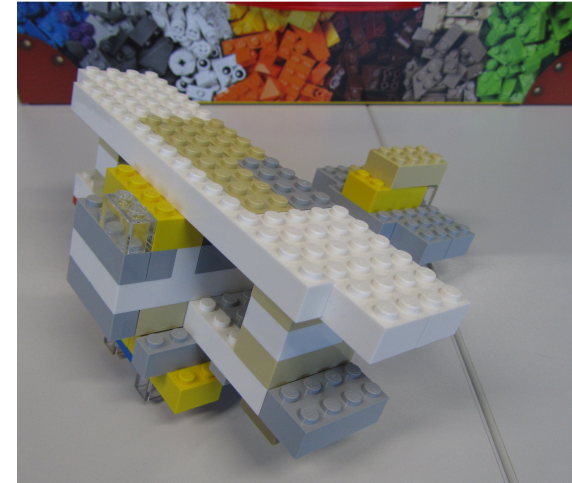
Toyplane, Resolution 20, Shell 2 Photo: © Institute of Applied Geometry, University Linz, Austria
