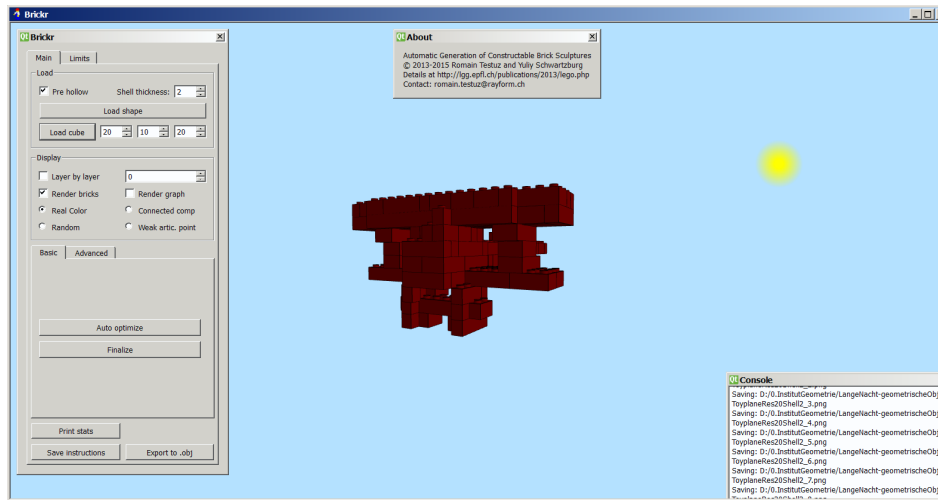
Toyplane, Resolution 20, Shell 2 Photo: © Institute of Applied Geometry, University Linz, Austria
