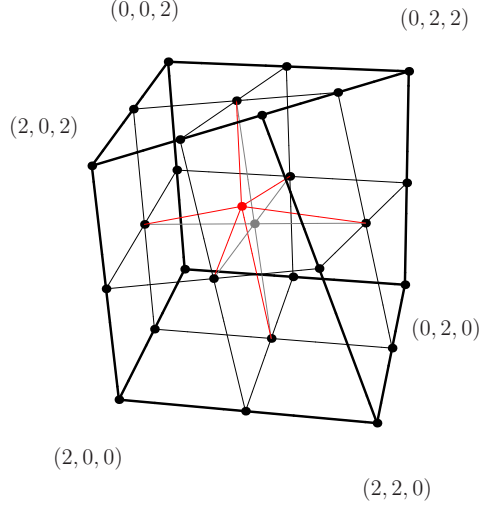
Figure 5: Control point grid for type V3. Only indices of selected control points are shown.
