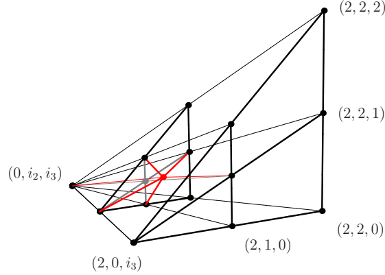
Figure 4: Control point grid for type V2. Only indices of selected control points are shown.
